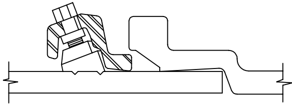
WEDGE DETAIL
