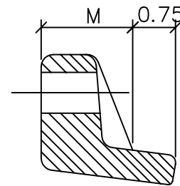
BOLT HOLE DETAIL
