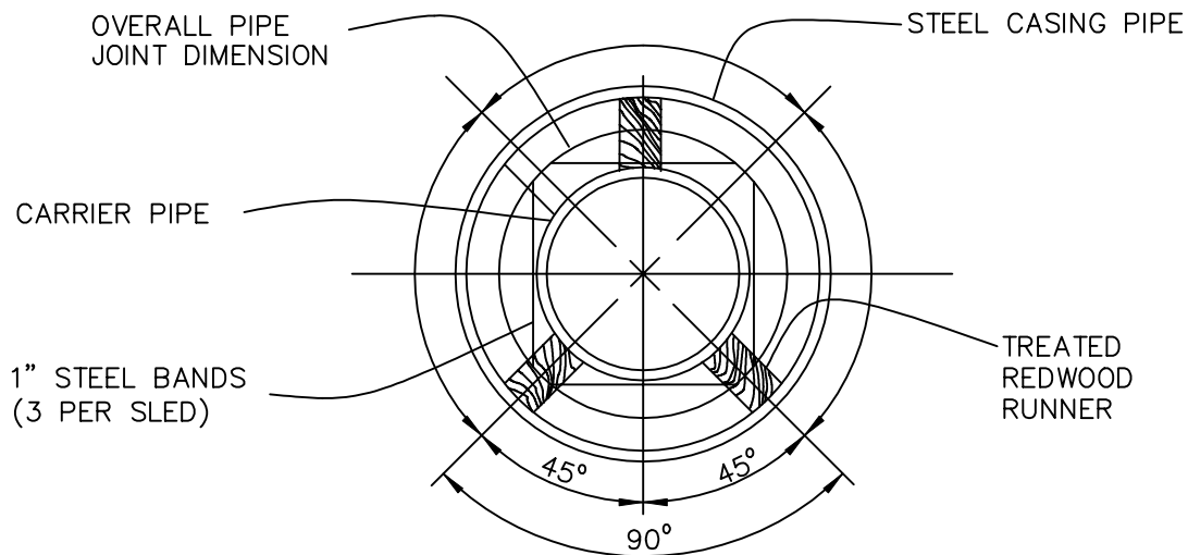
PIPE CASING DETAIL
