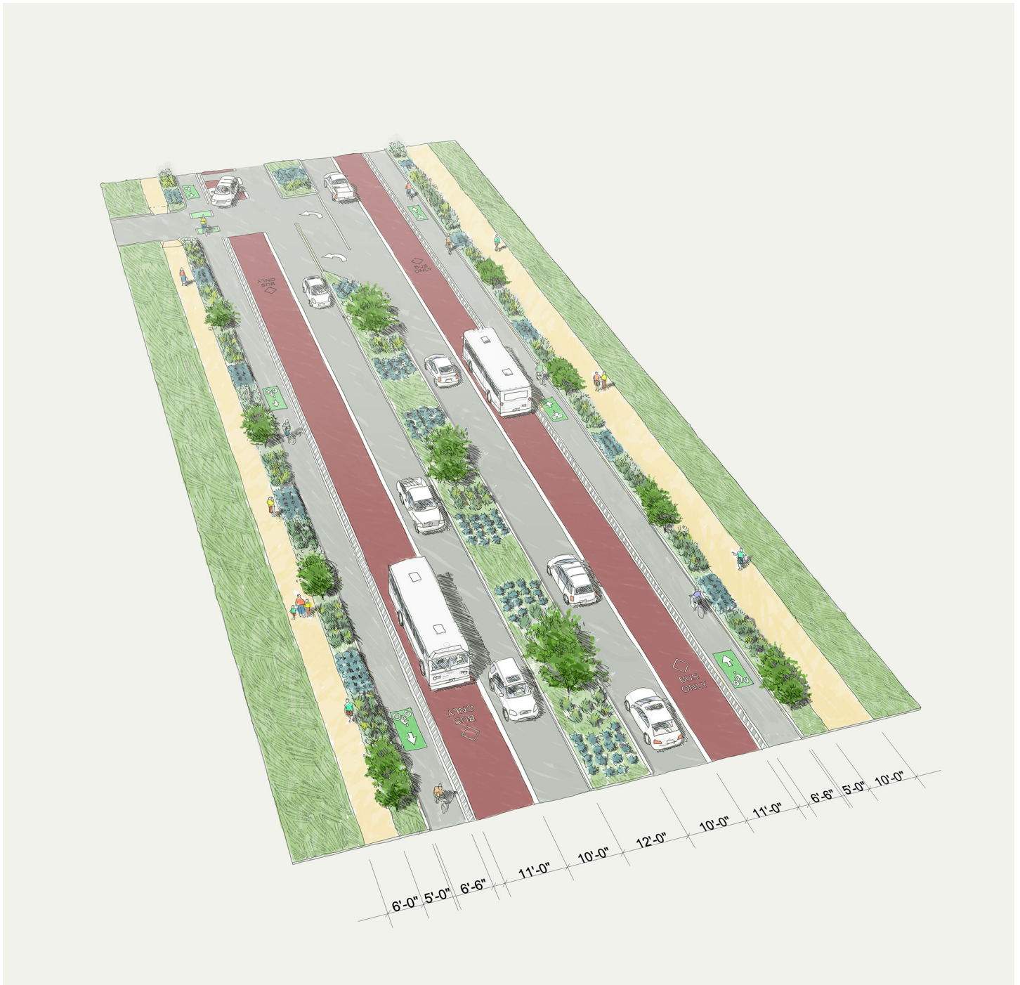
Figure H-11 District E - Alt 3 Side-Running BRT with Street-level Protected Bike Lane and Multi-Use Path (E.3.4)
