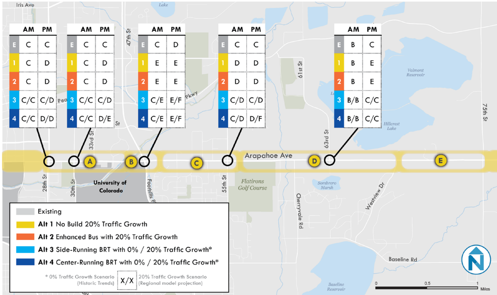
Figure A-4 Auto Level of Service, Peak Hour, All Directions, 2040
