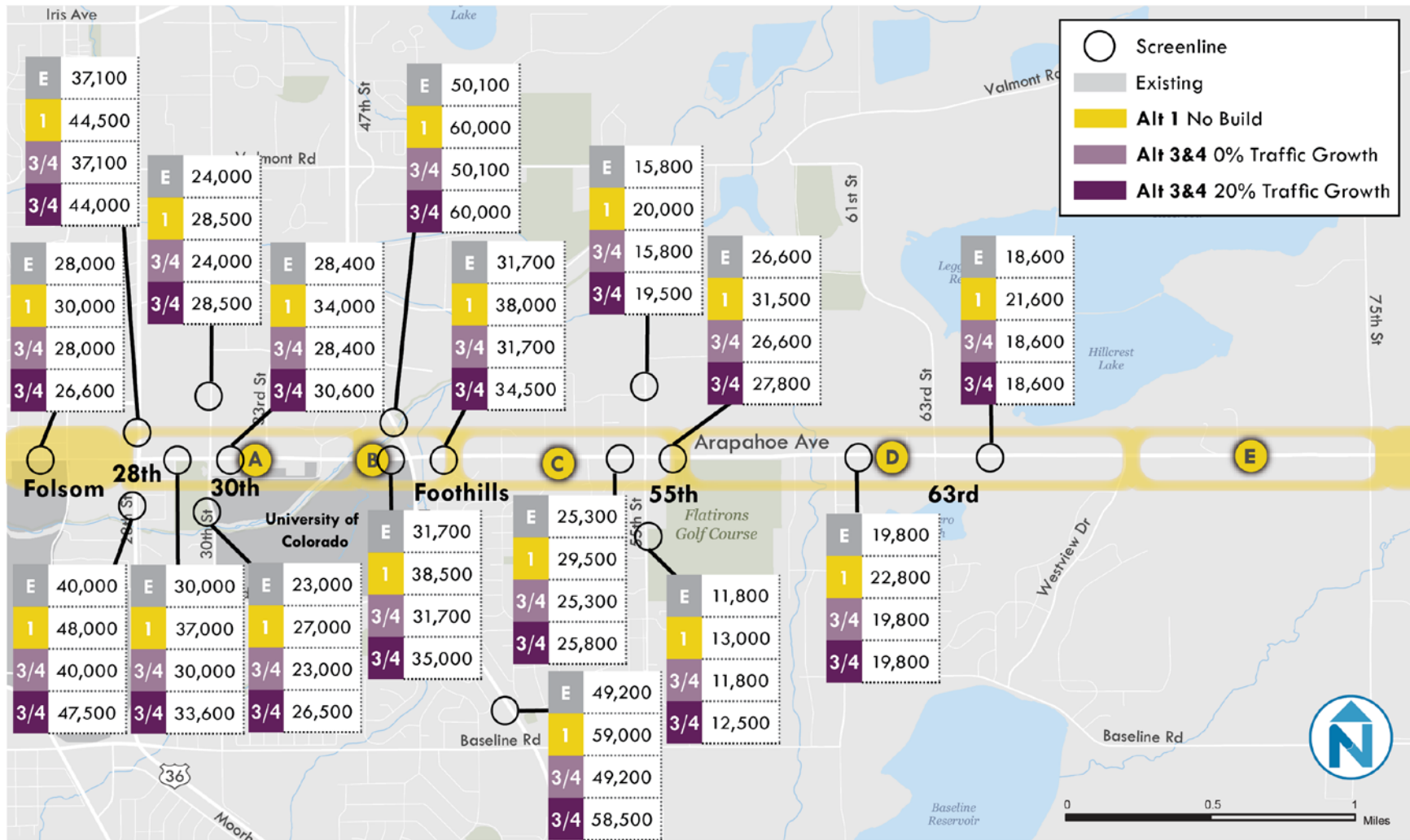
Figure A-6 Auto Volumes, Average Daily, Folsom to 75th Streets, 2040
