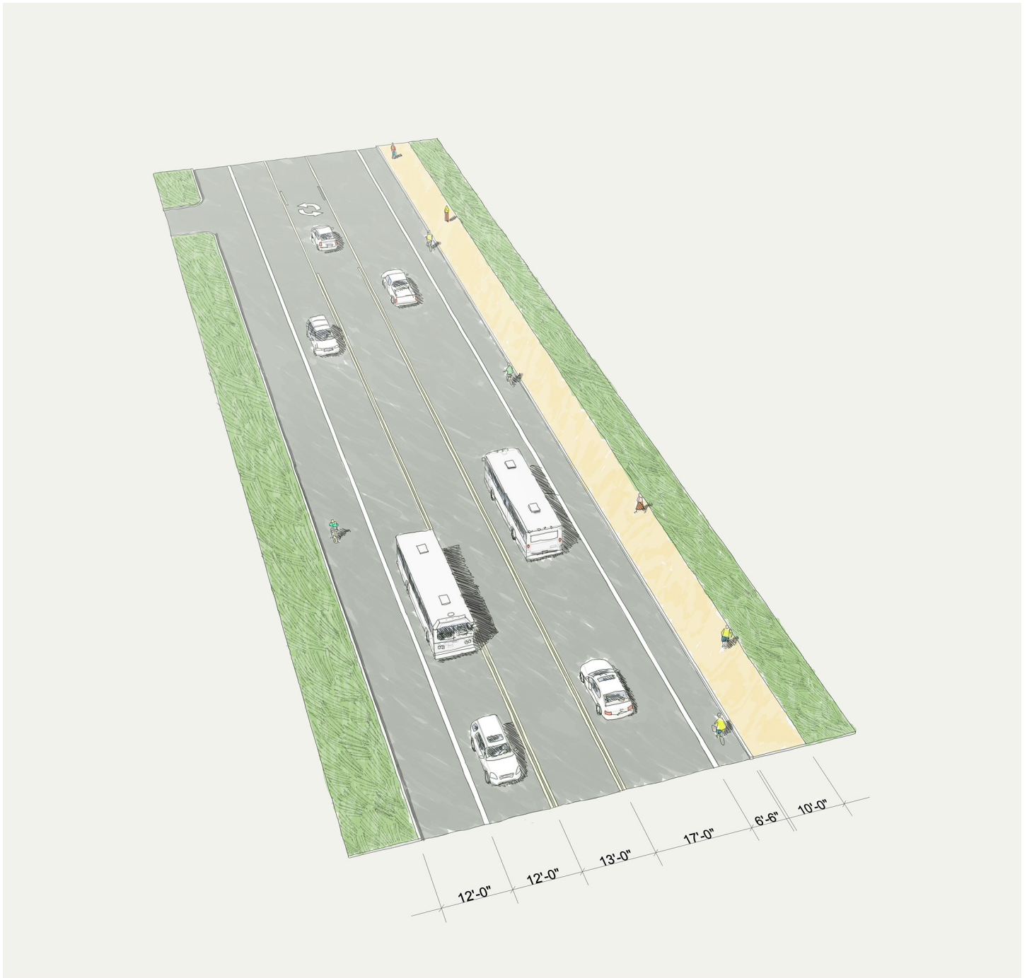
Figure H-9 District E - Alt 1 No Build with Existing Bike Lane and/or Multi-Use Path (E.1.0)
