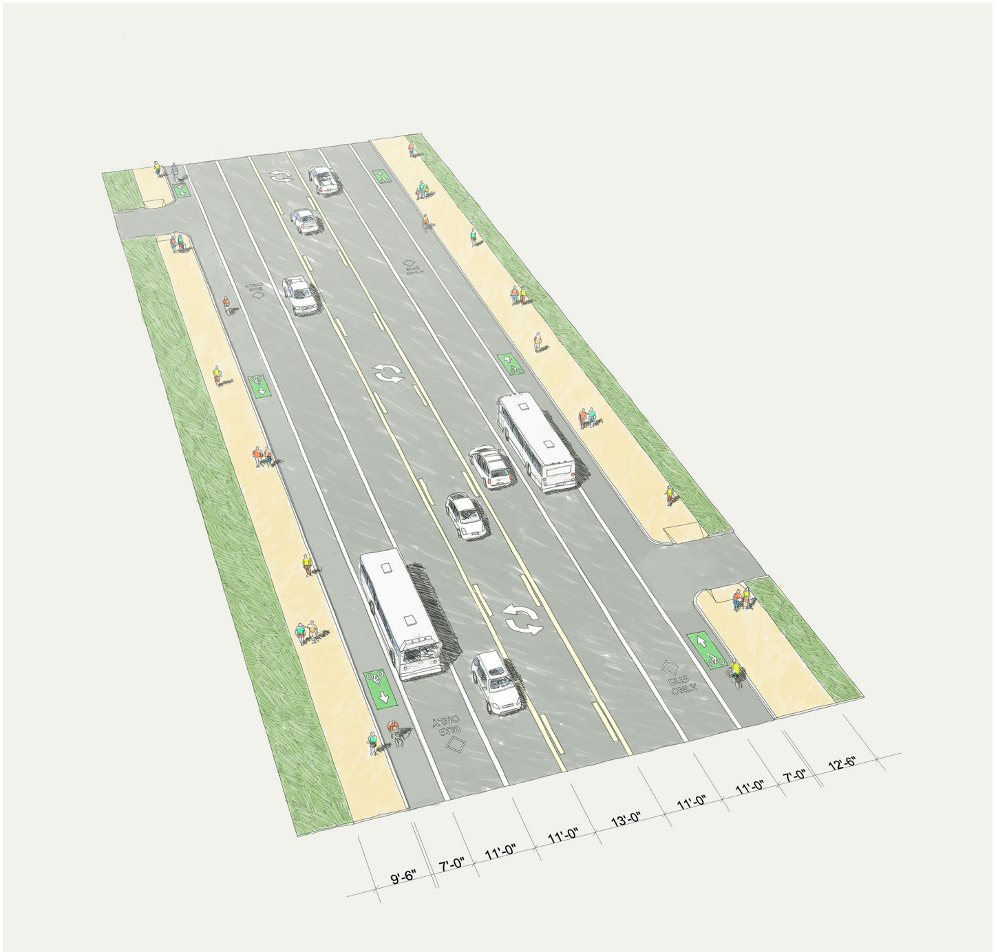
Figure H-7 District D - Alt 1 No Build with Multi-Use Path (D.1.0)
