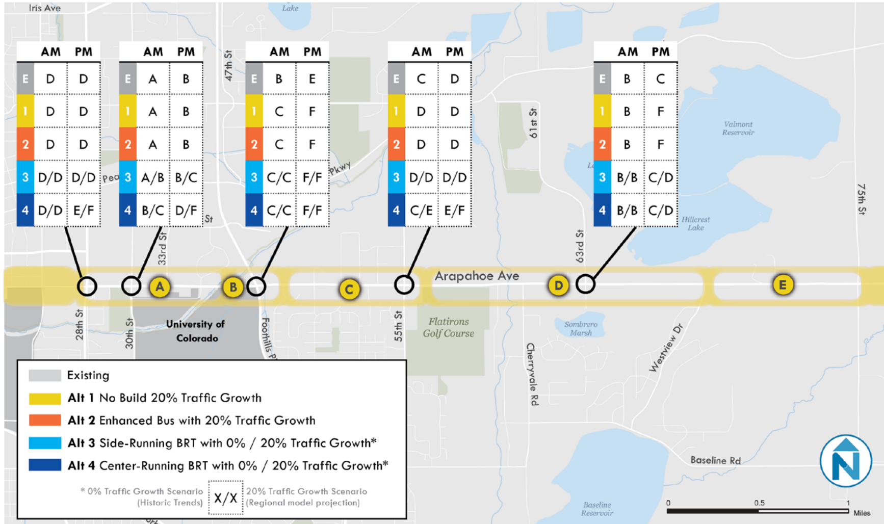
Figure A-5 Auto Level of Service, Peak Hour, East-West Peak Direction Only, 2040
