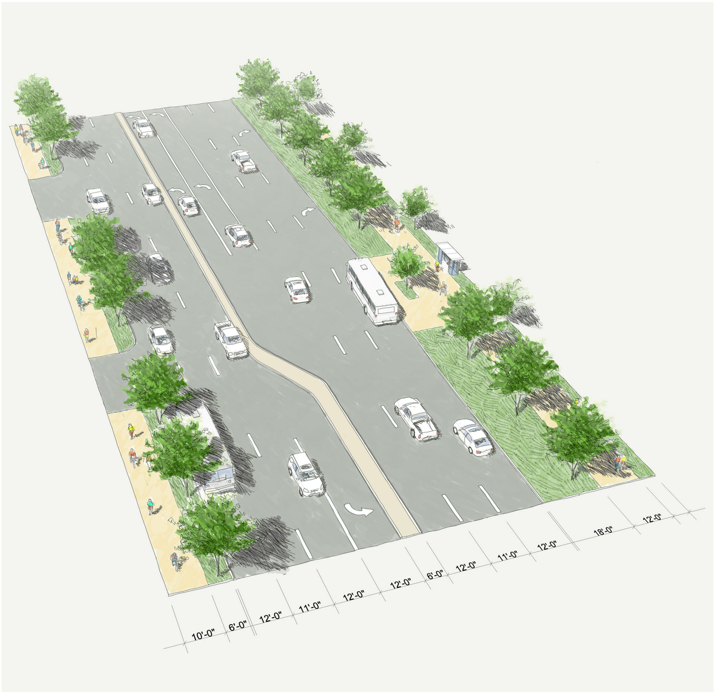
Figure H-2 District A - Alt 1 No Build with Multi-Use Path (A.1.0)
