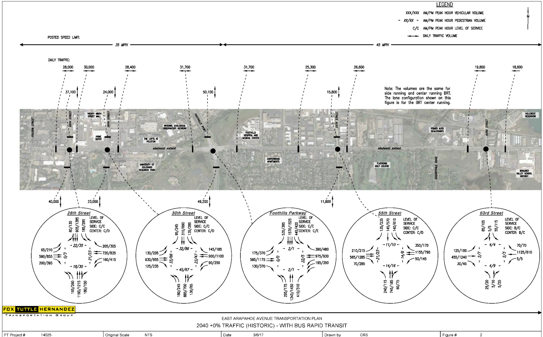
Figure A-9 Alts 3 and 4 (BRT) 2040 Vehicle Volumes and Level of Service at Key Intersections with 0% Traffic Growth
