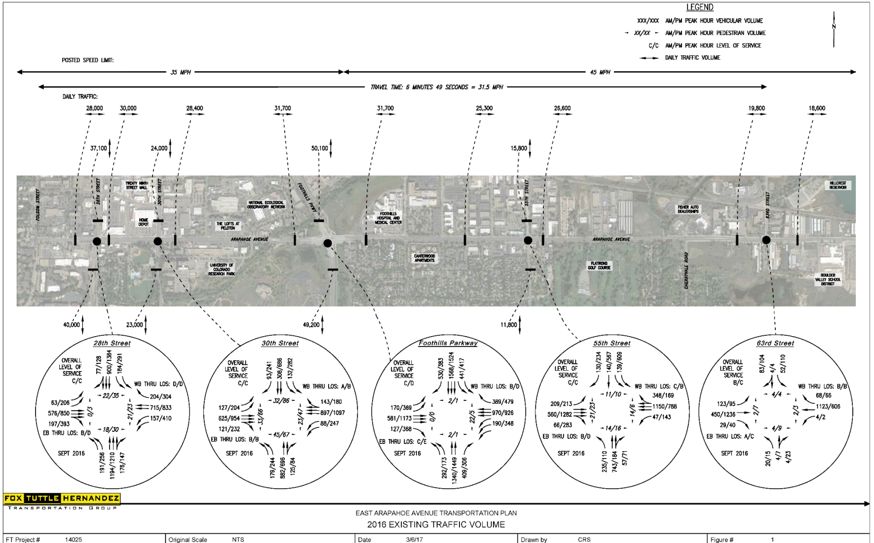
Figure A-7 Existing Vehicle Volumes and Level of Service at Key Intersections
