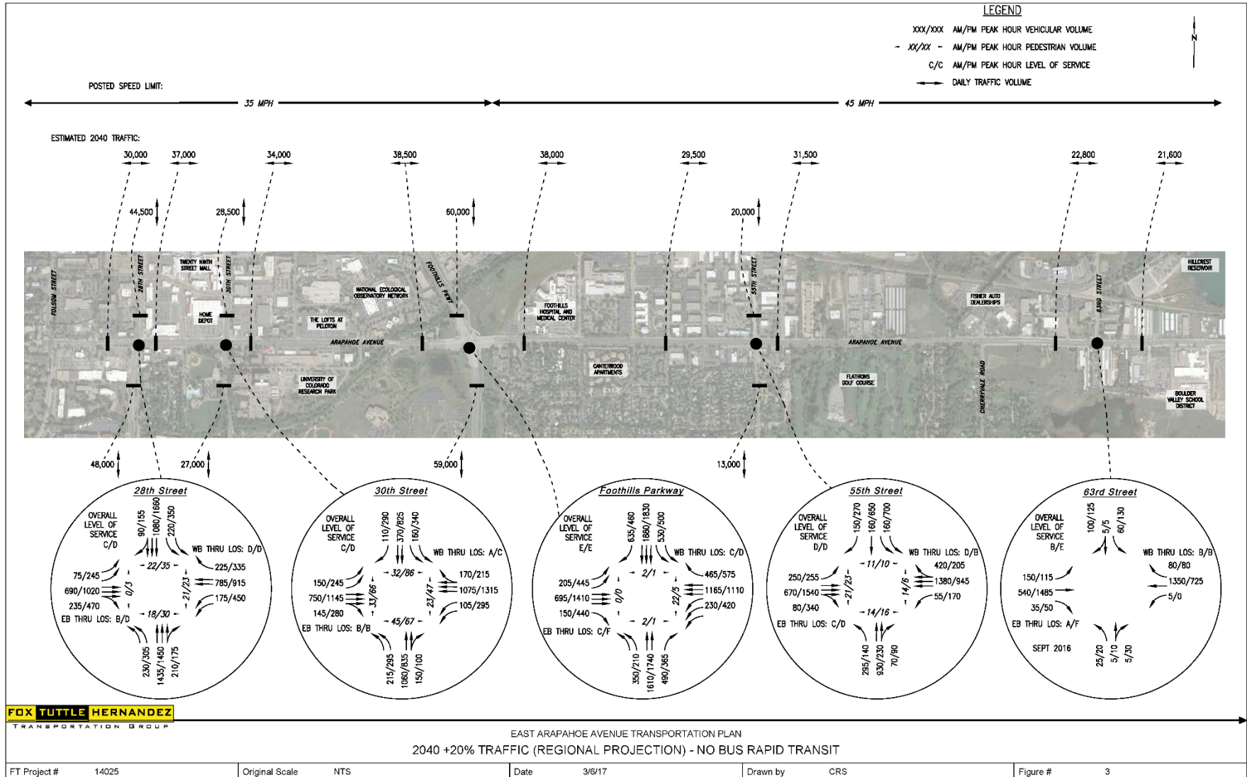
Figure A-8 No Build 2040 Vehicle Volumes and Level of Service at Key Intersections with 20% Traffic Growth
