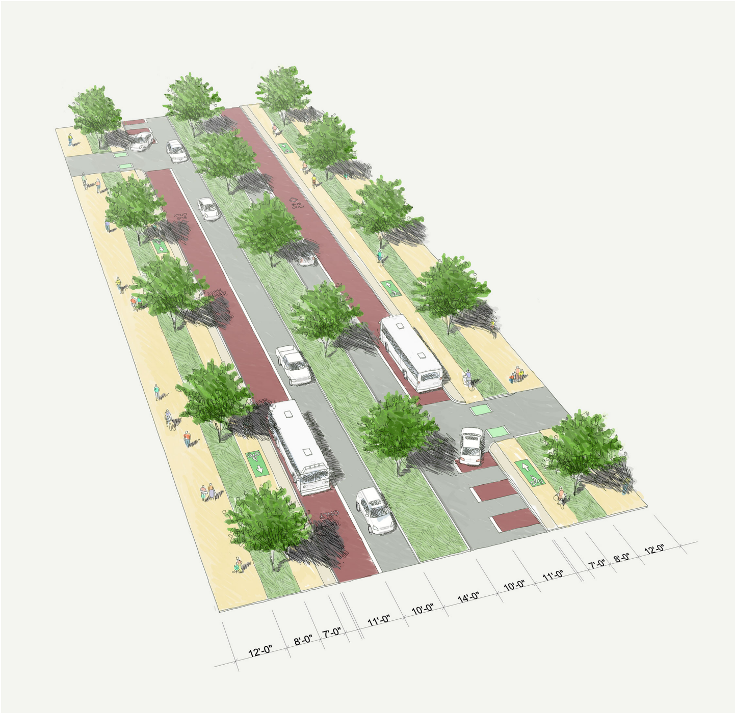
Figure H-8 District D - Alt 3 Side-Running BRT with Raised Protected Bike Lane and Multi-Use Path (D.3.1a)
