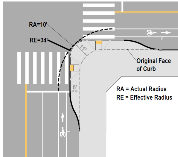
Figure 2. Actual and Effective Radius At An Intersection Corner With A Curb Extension
