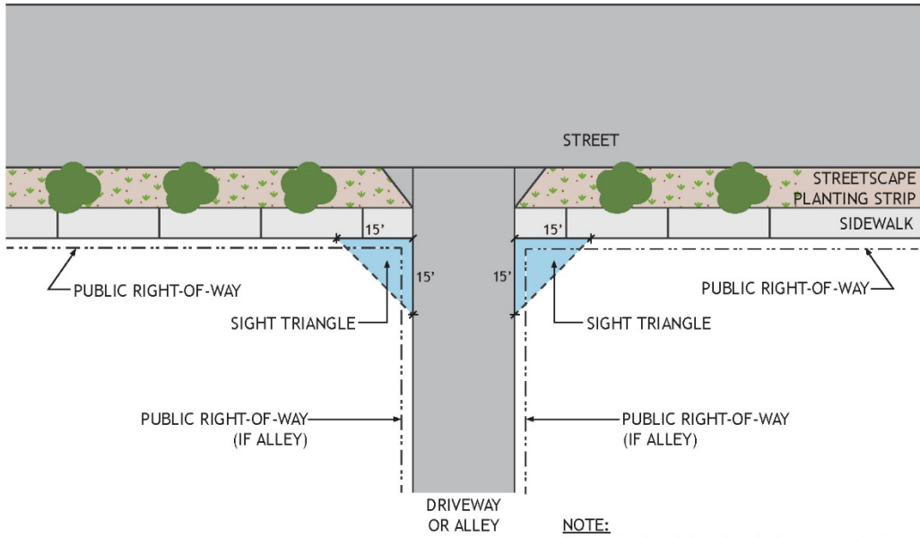
SIGHT TRIANGLES AT THE INTERSECTION OF A DRIVEWAY OR ALLEY WITH A SIDEWALK ON A PUBLIC STREET
