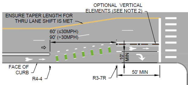
BIKE/TURN LANE - EXCLUSIVE TREATMENT (NO PARKING)
