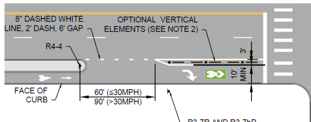
BIKE/TURN LANE - MIXING ZONE TREATMENT (NO PARKING)
