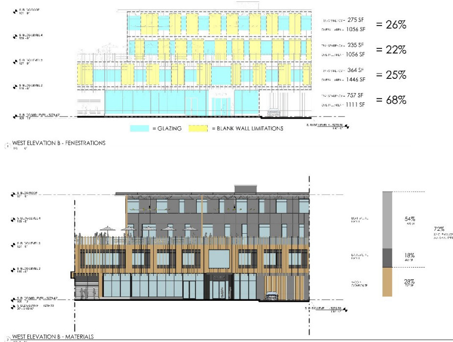
Figure 1: Example of fenestration pattern per floor, and percentage and type of materials
